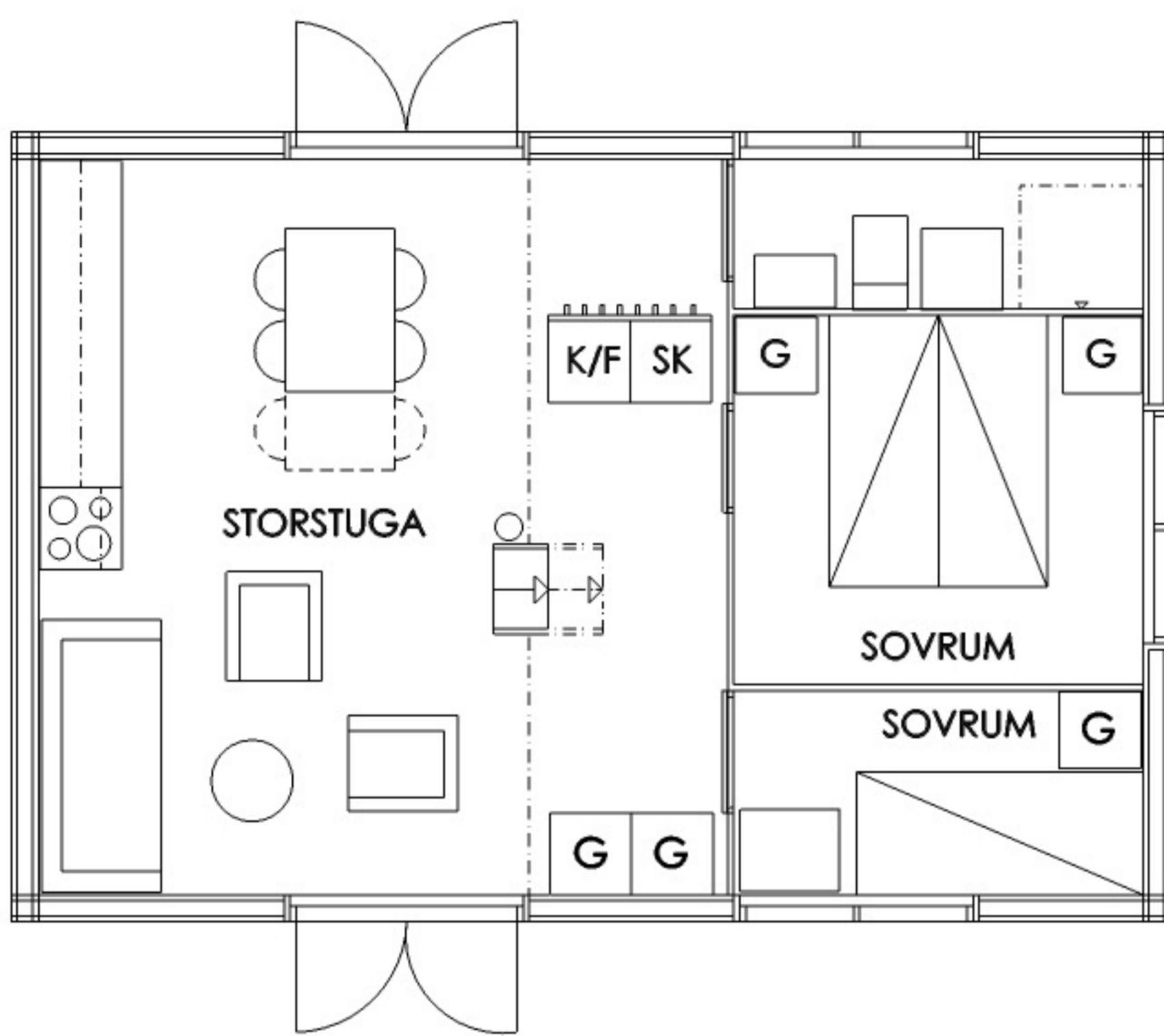
BOTTENPLAN
